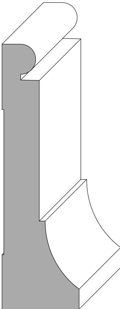
C536 1-5/16" x 4-1/2"
