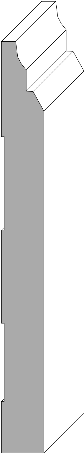
B548 3/4" x 7-1/4"
