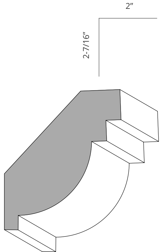
CR536 1-1/16" x 3-1/8"
