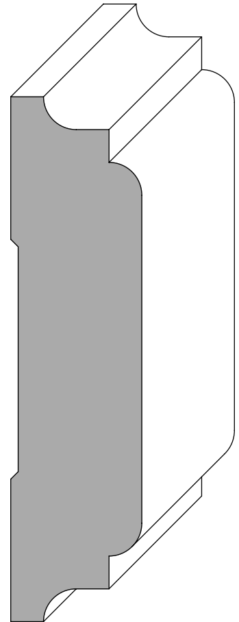
CHR365 1" x 4"
