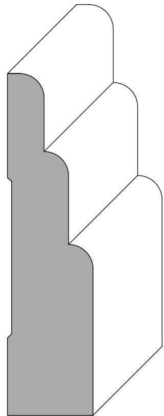
C563 7/8" x 3-1/2"
