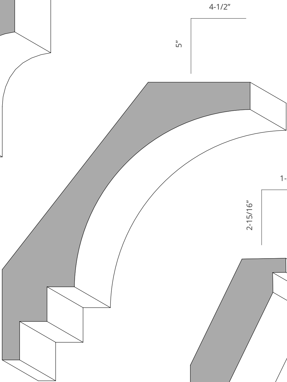
CR527 1-3/4" x 6-11/16"
