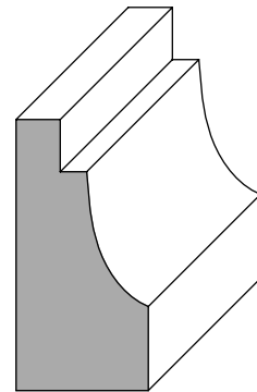
PA52 5/8" x 1-5/16"
